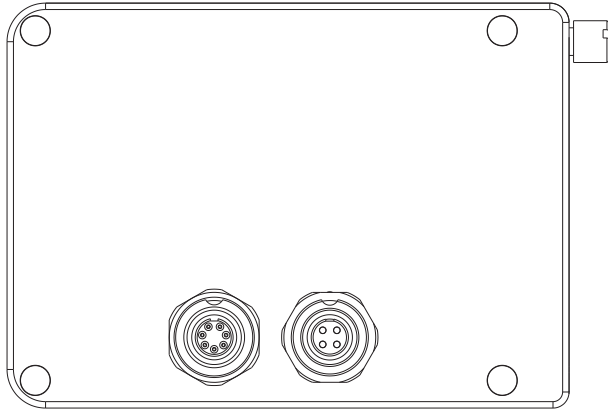
7 pin female connector - pinout external view
