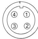
4 pin female connector - pinout external view
