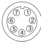
7 pin female connector - pinout external view
