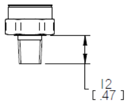
Binder connector – Harness side
